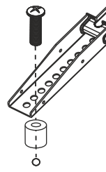
M5x25 (B)
