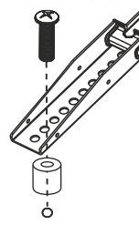
M5x25 (B)
